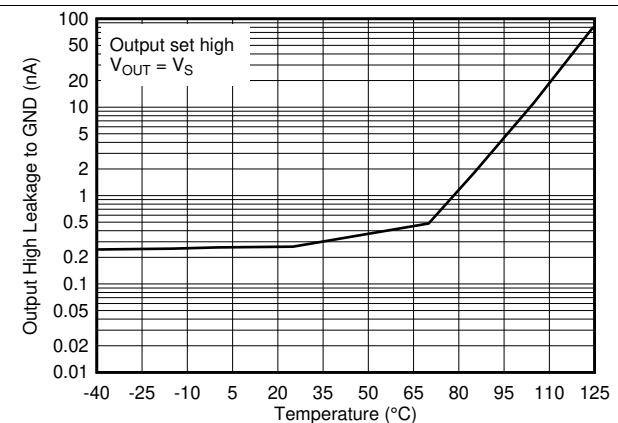
Figure 29. Output High Leakage Current vs. Temperature at 36V
