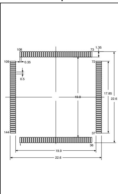
Figure 77. Recommended footprint (1)(2)
