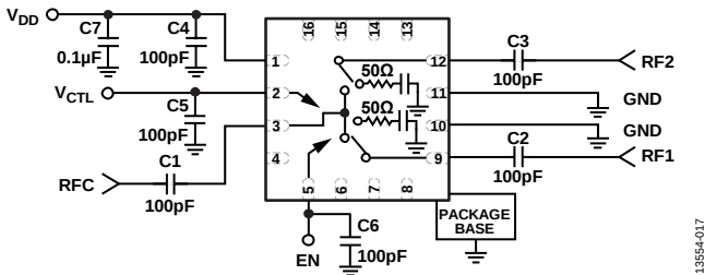
Figure 17. HMC8038 Application Circuit
