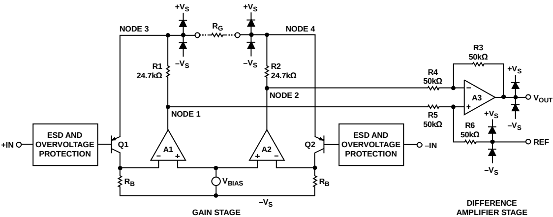
Figure 58. Simplified Schematic
