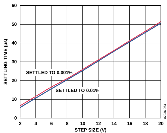
Figure 56. Settling Time vs. Step Size, V_S = \pm 15\text{V} Dual Supplies
