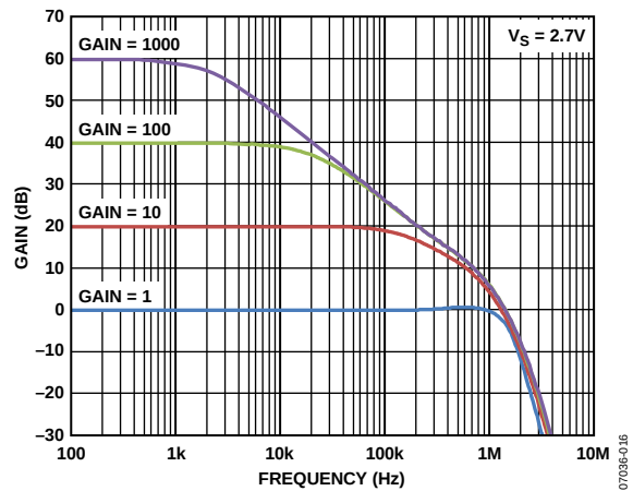
Figure 26. Gain vs. Frequency, 2.7\text{ V} Single Supply
